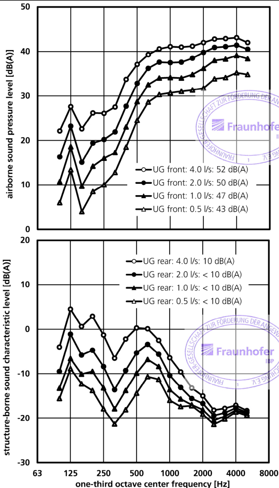
Frequency spectrum of the airborne sound pressure level L_{p,A} (above) and structure-borne sound characteristic level L_{sc,A} (below) measured at various flow rates according to DIN EN 14366 . Test specimen: Wastewater system made of plastic "Kalde Mute FR" with fittings "Kalde, PVC-U, S14" (manufacturer: Kalde Klima A.Ş.) and acoustic pipe clamps "Bismat 1000" (manufacturer: Walraven). Further information on the test setup can be found in the results sheet 1 as well as figures 4 and 5.
